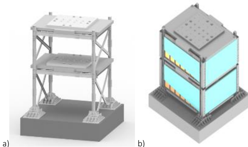
Figure 1. FUTURE mock-up; overall layout without (a) and with cladding (b)
